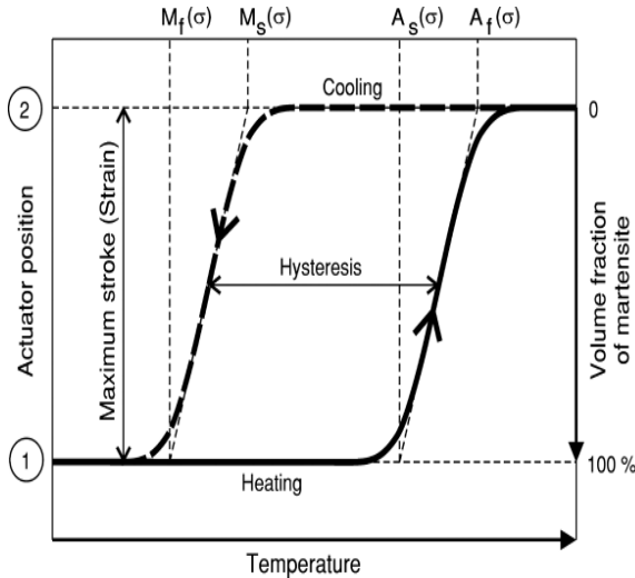
Fig1. Temperature – induced phase transformation
