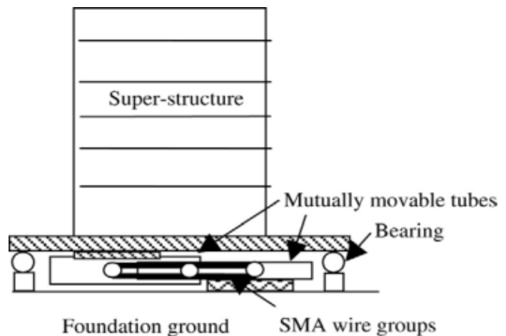
Fig10. SMA isolation system for buildings
