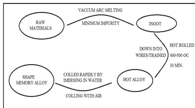
Fig3. Flow Chart Of Manufacturing
