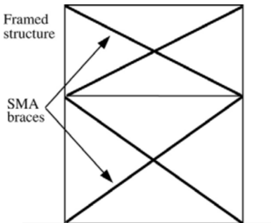
Fig9. SMA braces for a two-story steel frame
